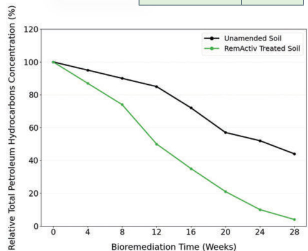
Figure 1: RMIT University study showing a 50% increase in degradation of TPH using RemActiv™ vs natural attenuation
