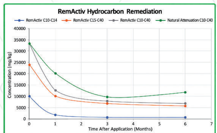
Figure 1: Degradation rates of Total Recoverable Hydrocarbons in contaminated soil following RemActiv™ treatment
